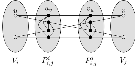
Figure 1: An illustration of the gadget construction in the proof of Theorem 3.3.
