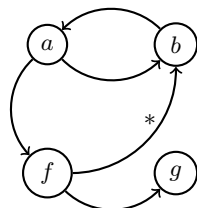
Fig. 1. Marked dependency graph of a CoLP P
